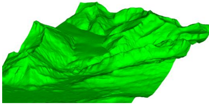
Fig. 2: LiDAR Data Distinguishes between Vegetation and Bare Earth, Enabling an Understanding of Vegetation Cover and Tree Canopy Height
